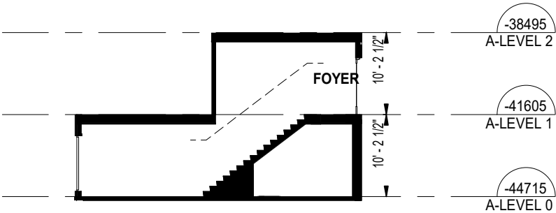
UNIT 010 - SECTION
